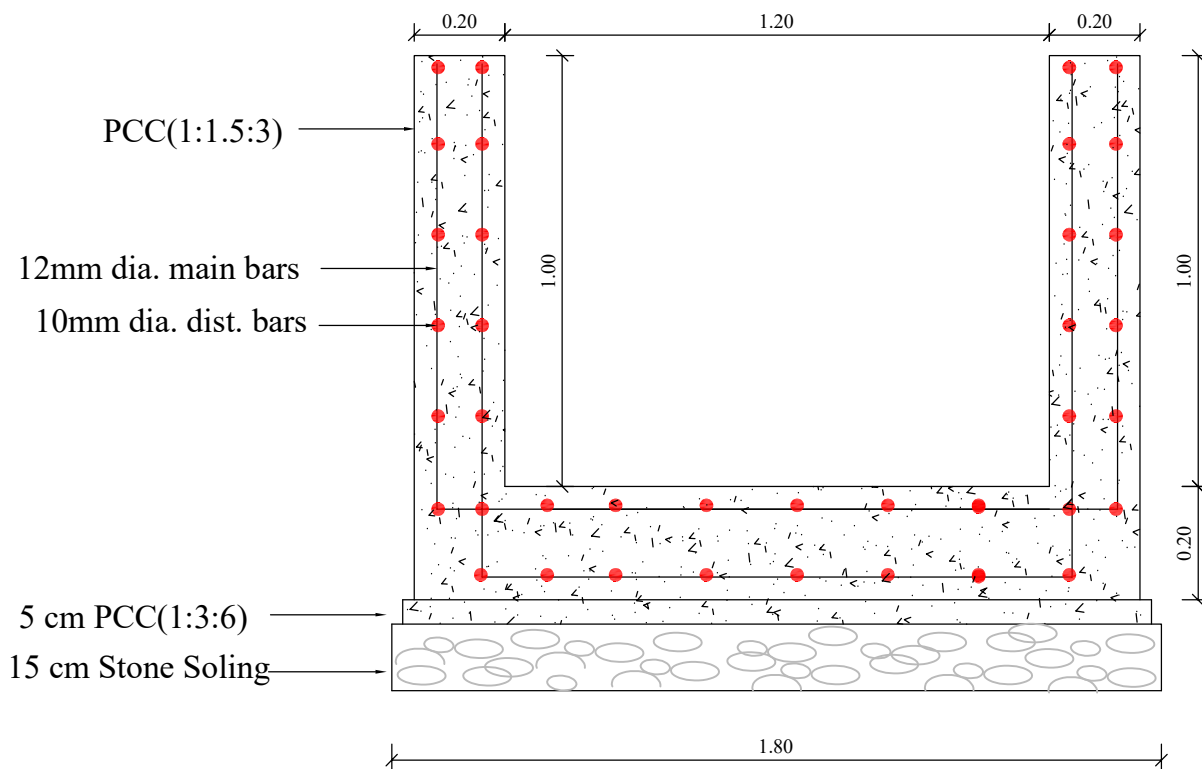
RCC Drain Wall Section
