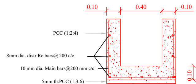
Main Canal Section
