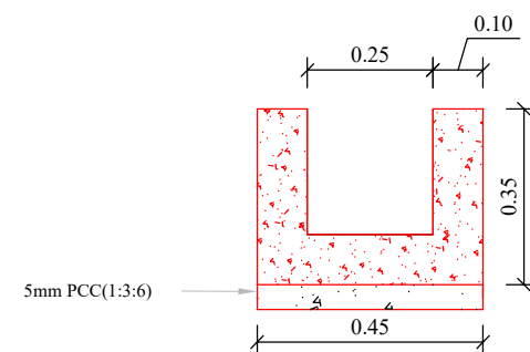
Branch Canal Section
